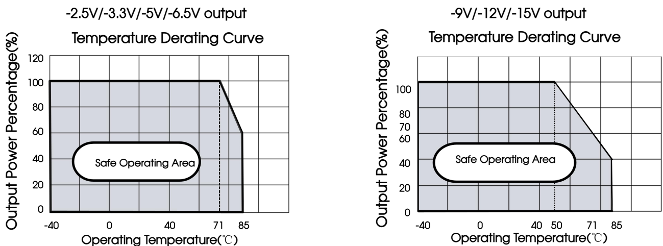
Fig. 1-③ Free air convection curve (Negative output)
