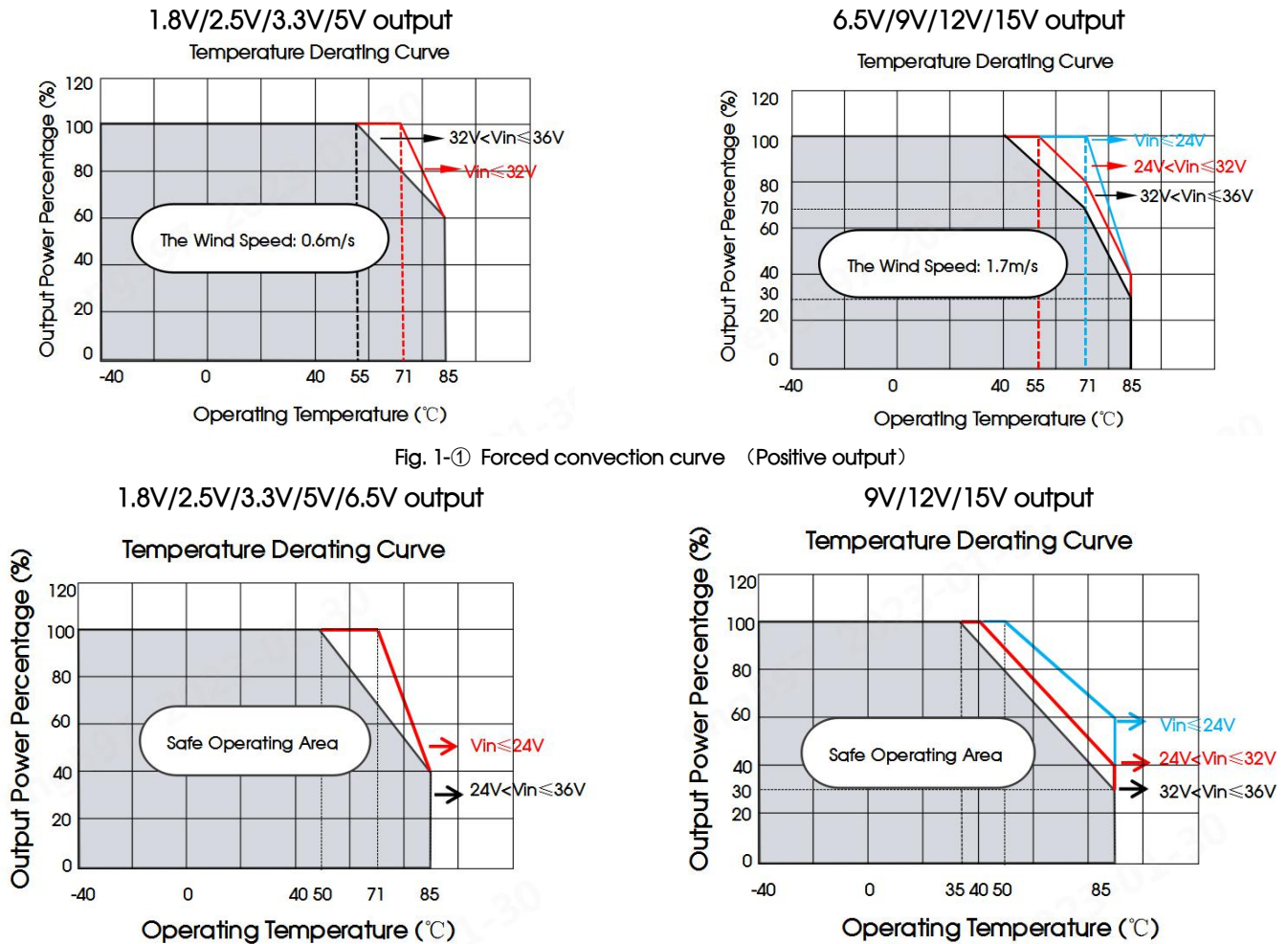
Fig. 1-② Free air convection curve (Positive output)
